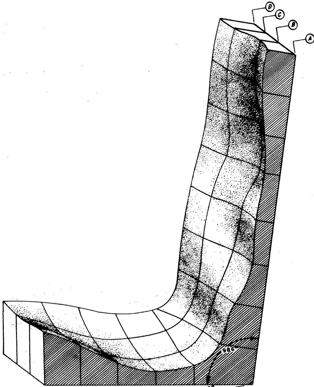
CHOICE COCKPIT AT 35 INCH LEVEL. MIDLINE SECTION OF SEAT CONTOURING (A) SHOWING PROFILES AT THREE INCH INTERVALS LATERALLY. (B, C, AND D)
