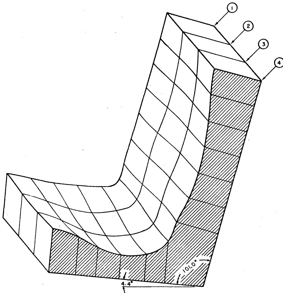
SEAT SECTION FOR 45" BOMBER COCKPIT, SHOWING PROFILES AT \epsilon (4) AND AT THREE INCH INTERVALS LATERALLY (3) - (2) & (1).
